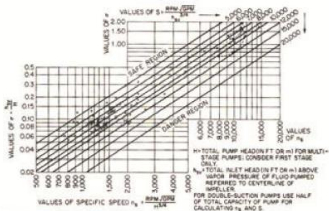
FIG. 31 Cavitation limits of centrifugal and propeller pumps. (Worthington Pump)
