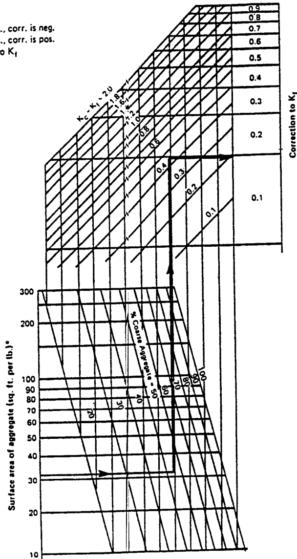
CHART FOR COMBINING K_f AND K_c TO DETERMINE K_m
