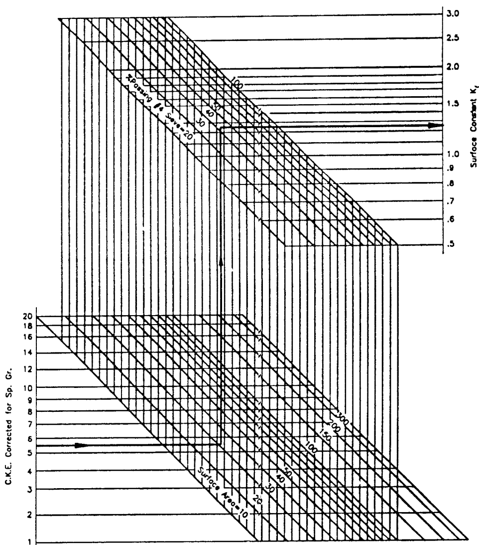
CHART FOR DETERMINING K FROM C.K.E.
